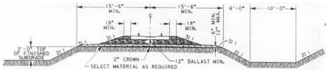
Figure 21: Typical Railroad Cross-Section
